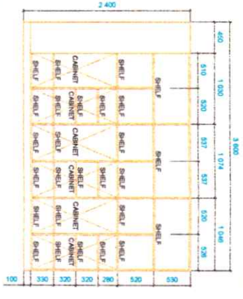
4 FRONT ELEVATION OF CABINET SCALE: AS SHOWN
