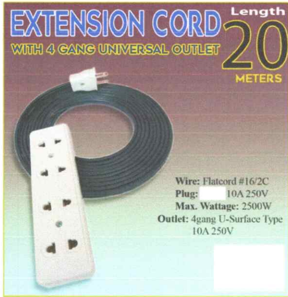
EXTENSION WIRE, 4 gang, at least 20 meters (item no. 178)
