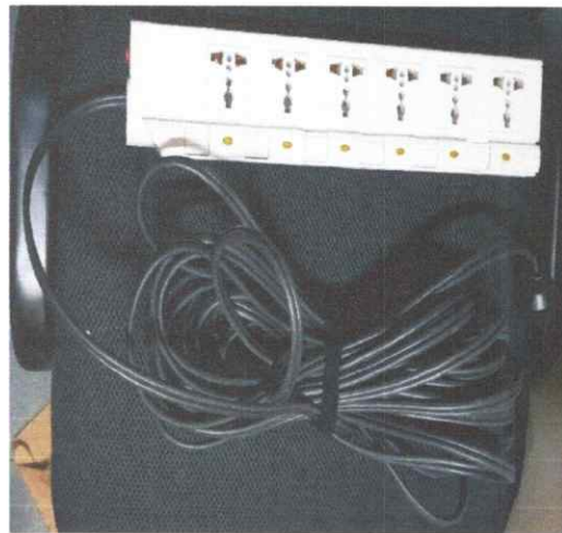
EXTENSION WIRE, 6 socket with universal outlet and individual switch, at least 15 meters (item no. 181)
