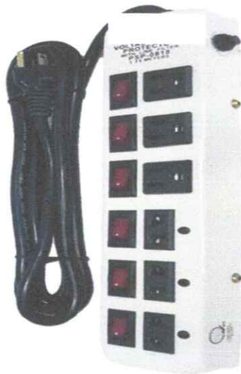
EXTENSION WIRE, 6 gangs with individual switch, at least 1.75 meters (item no. 180)
