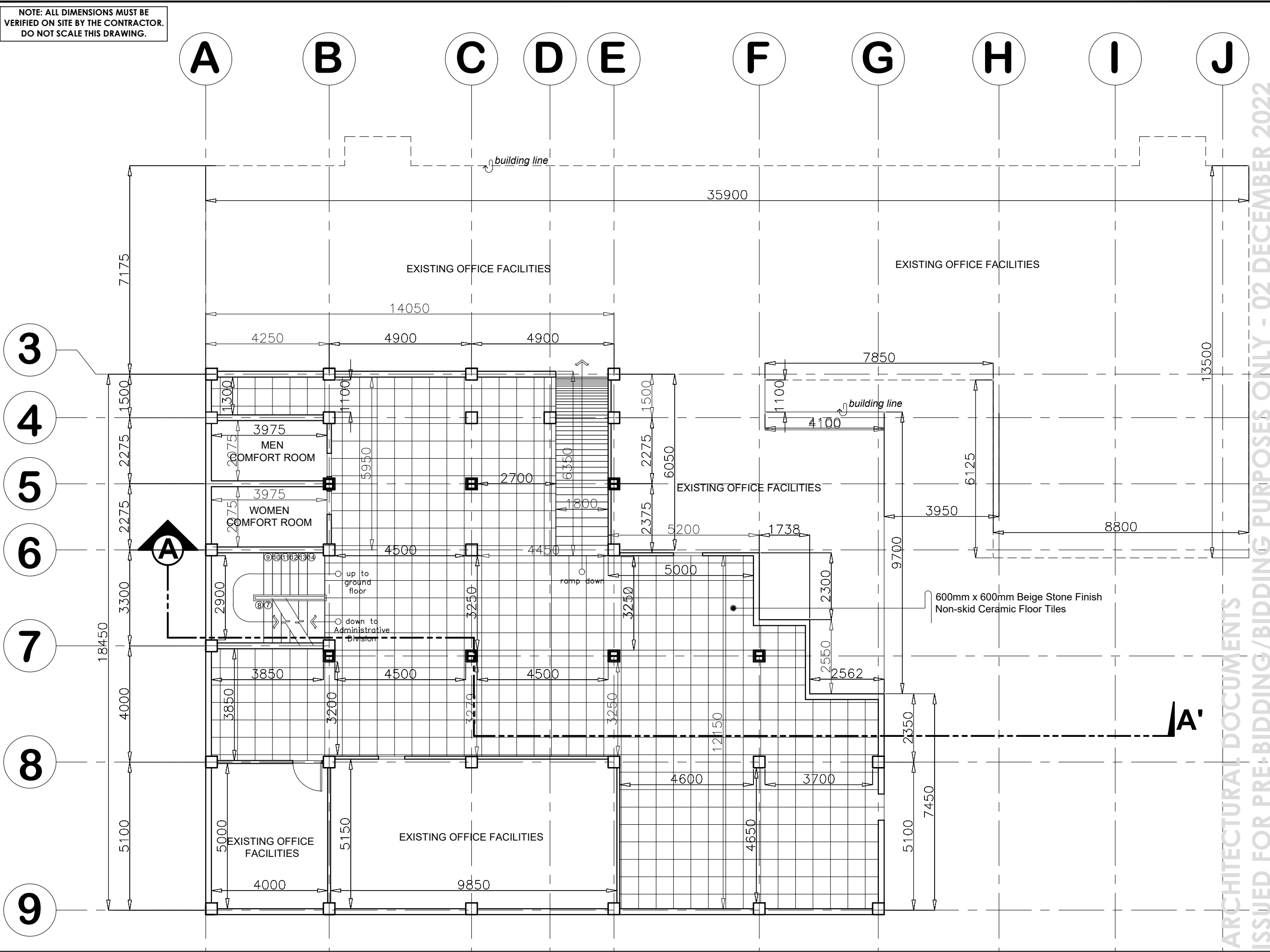
FIRST BASEMENT FLOOR DEMARCATION PLAN SCALE: 1:125 METERS
