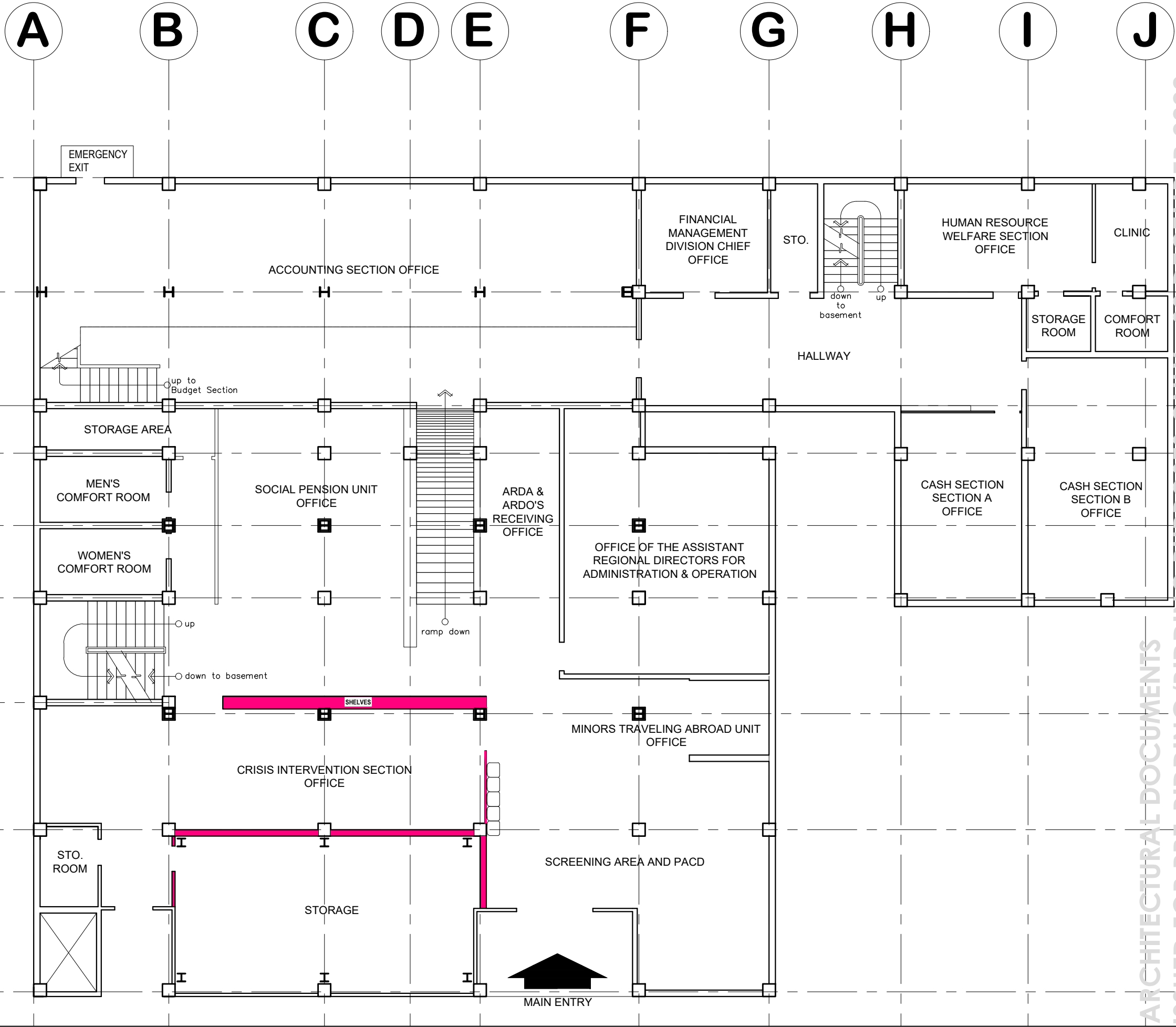
GROUND FLOOR DEMOLITION DEMARICATION PLAN SCALE: 1:125 METERS
