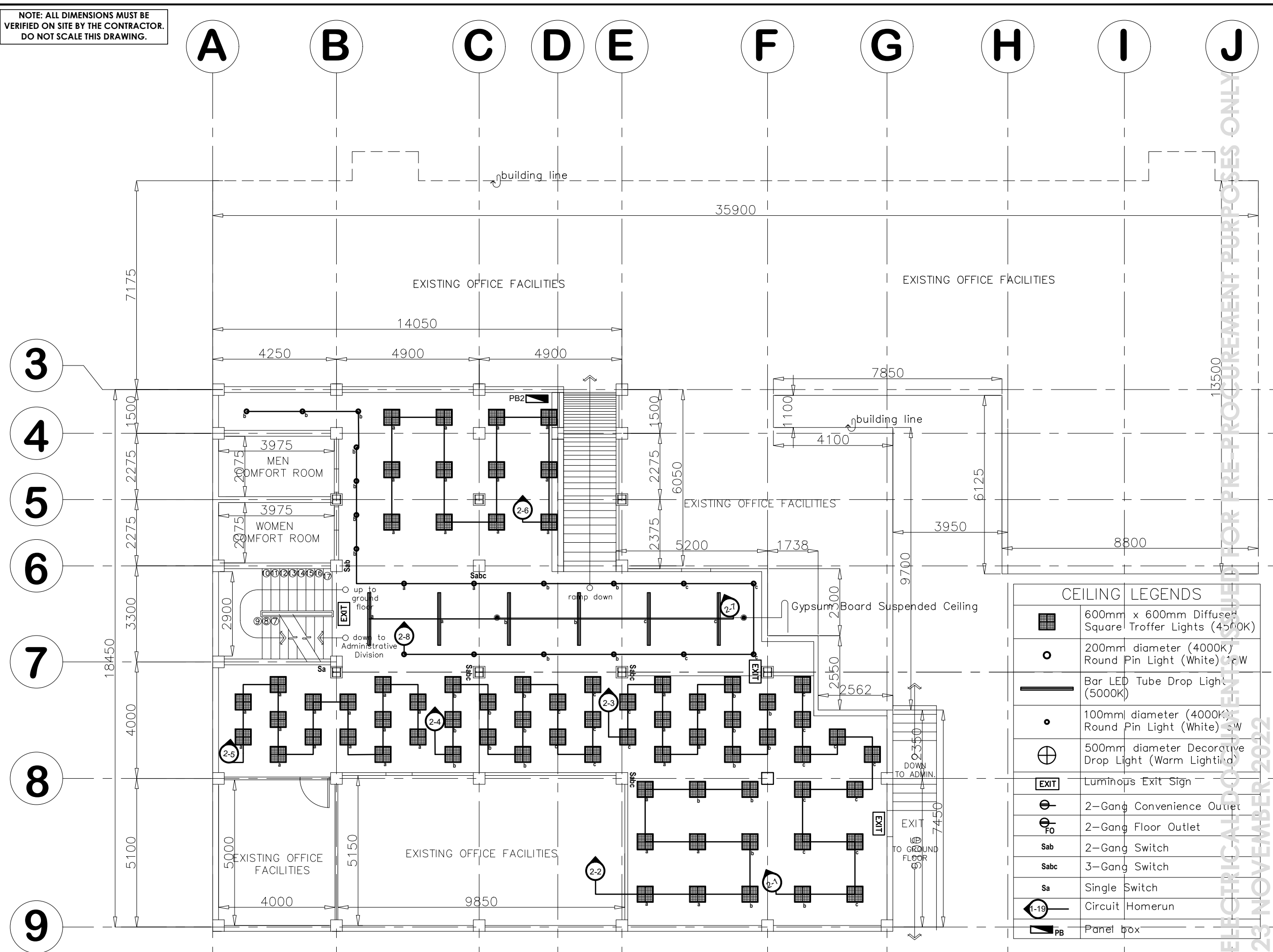
1 E 2 FIRST BASEMENT LIGHTING LAYOUT SCALE 1:125 METERS
