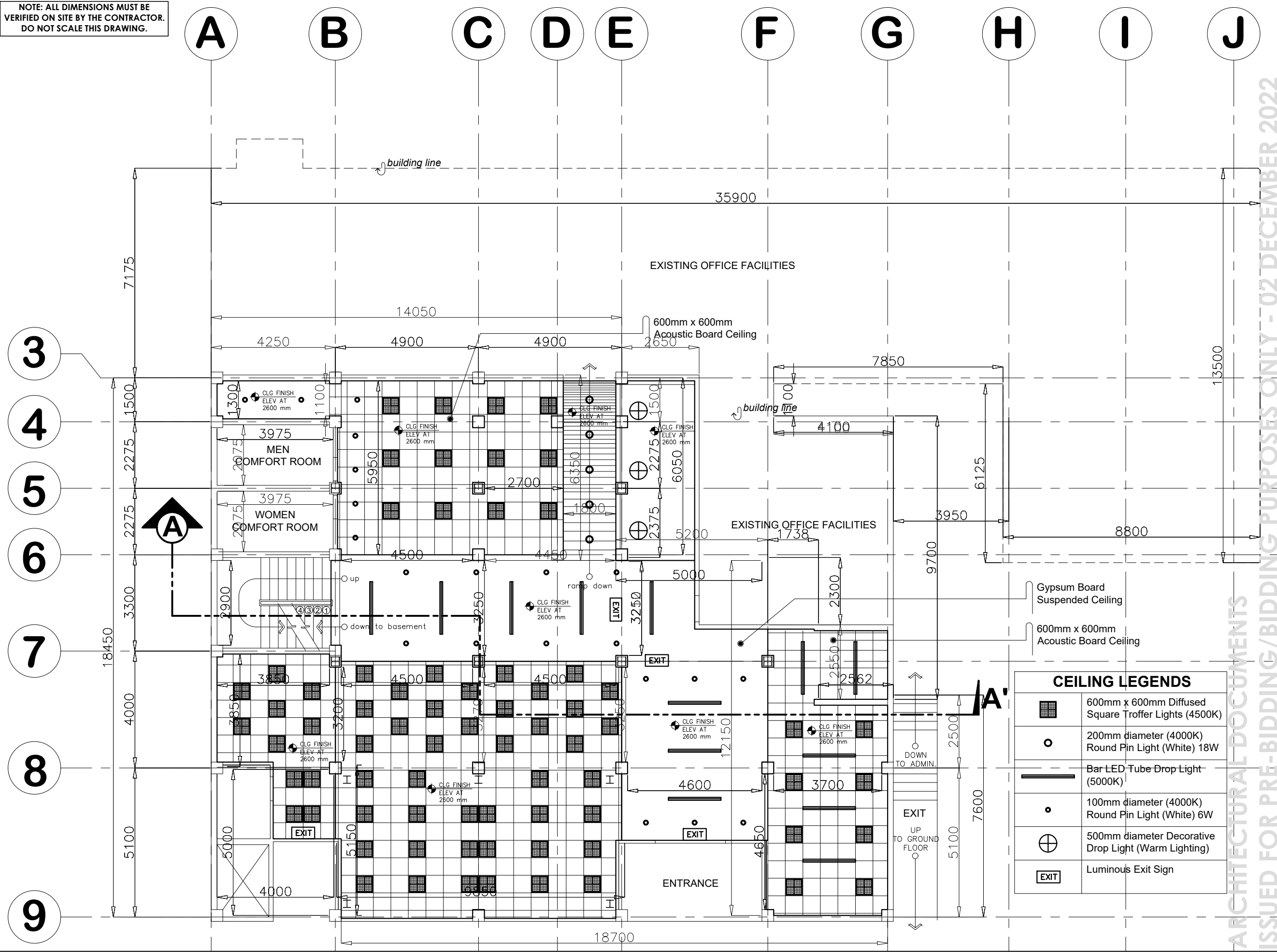
1 A 7 GROUND FLOOR REFLECTED CEILING PLAN SCALE: 1:125 METERS
