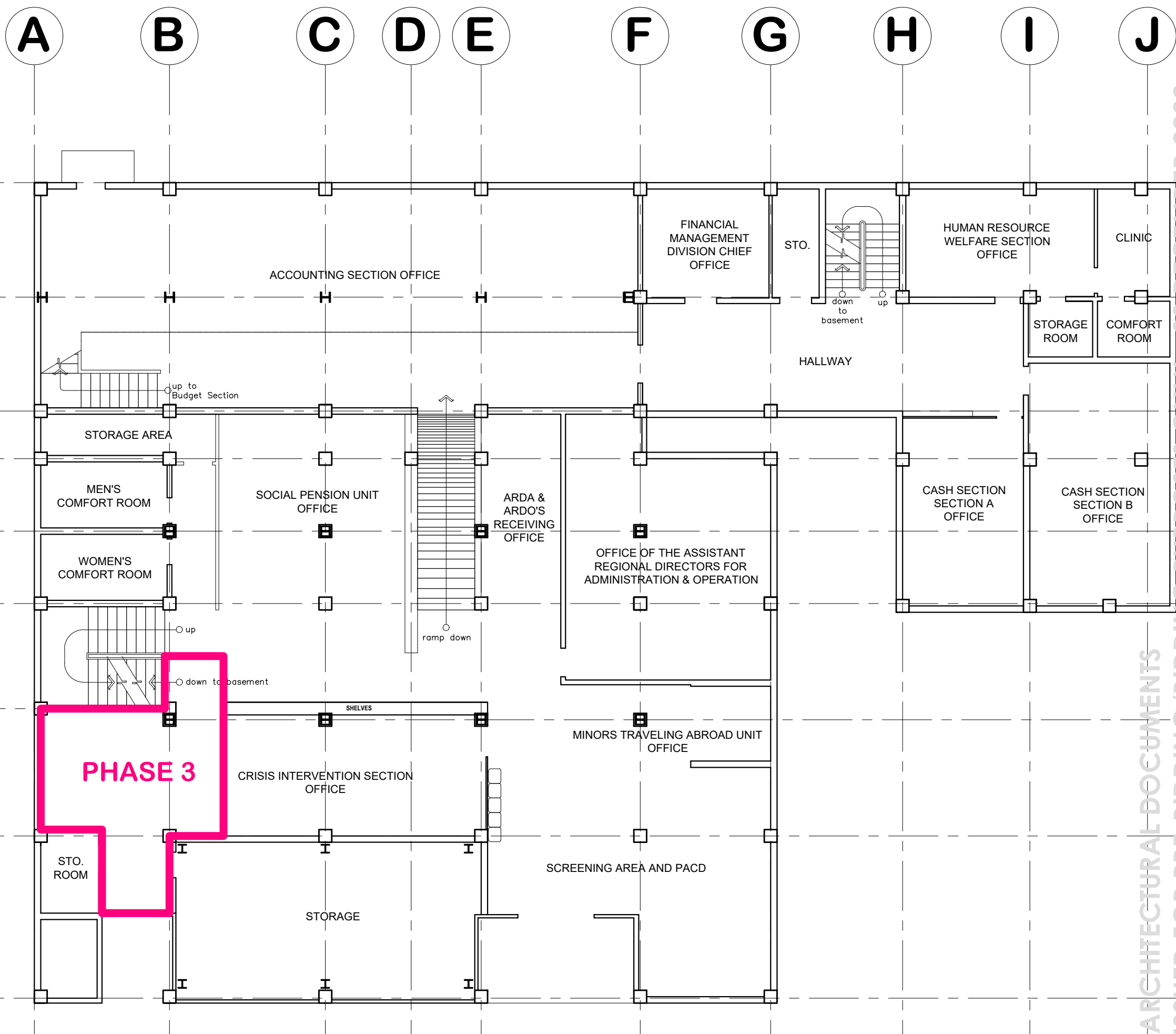
CONSTRUCTION PHASE 3 DEMARCATIION PLAN SCALE: 1:125 METERS
