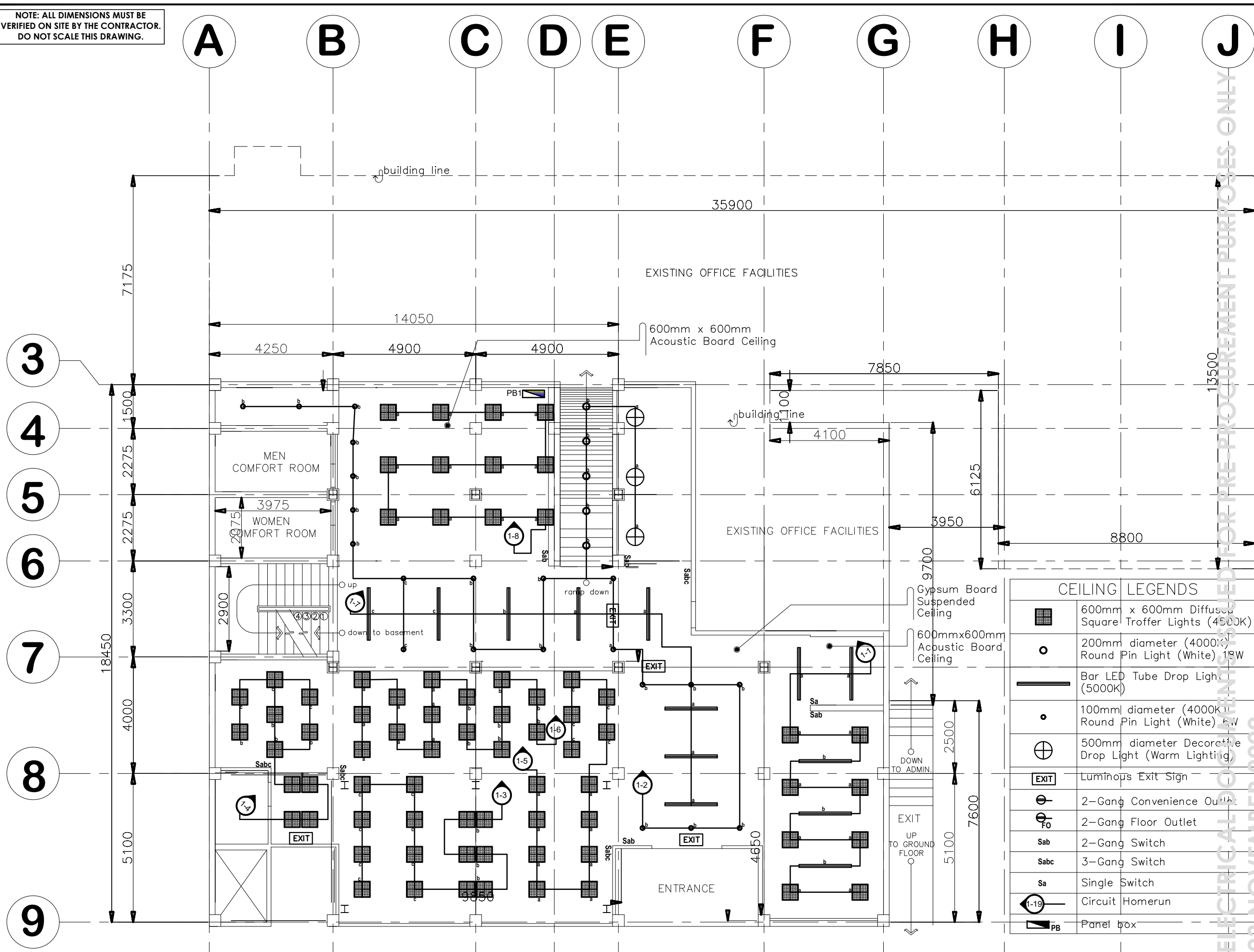
1 E 1 GROUND FLOOR LIGHTING LAYOUT SCALE 1:125 METERS
