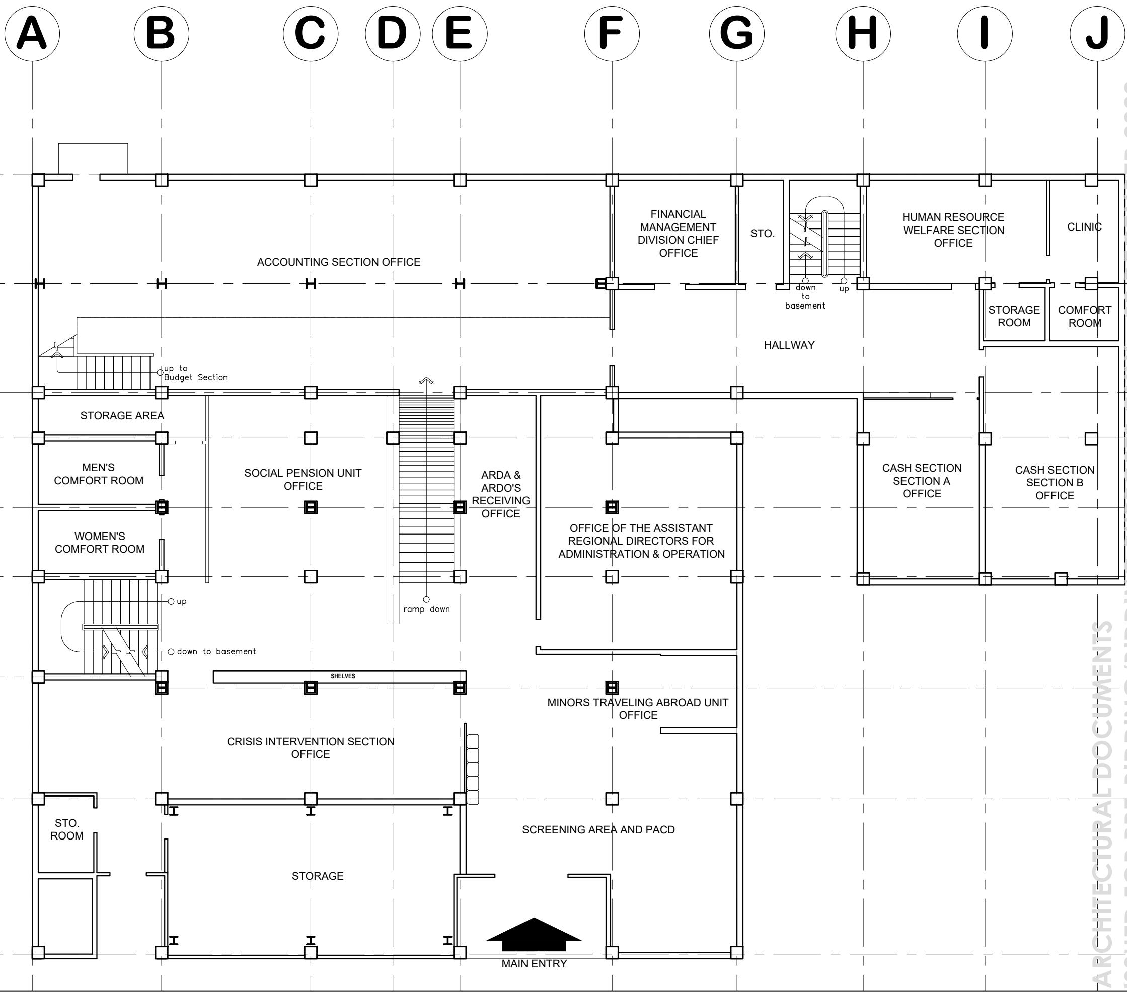
GROUND FLOOR BASE-BUILD PLAN SCALE: 1:125 METERS
