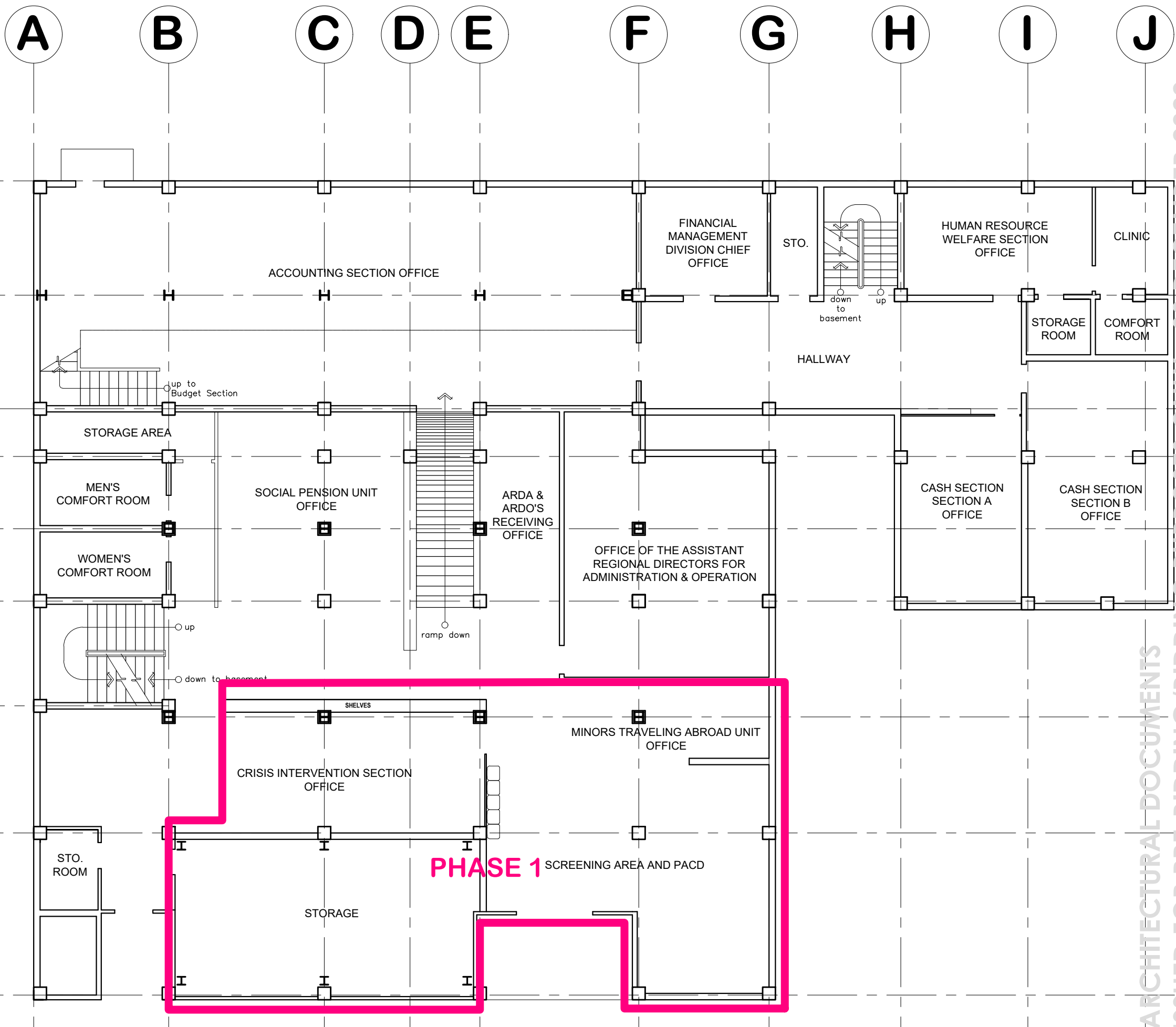
CONSTRUCTION PHASE 1 DEMARICATION PLAN SCALE: 1:125 METERS
