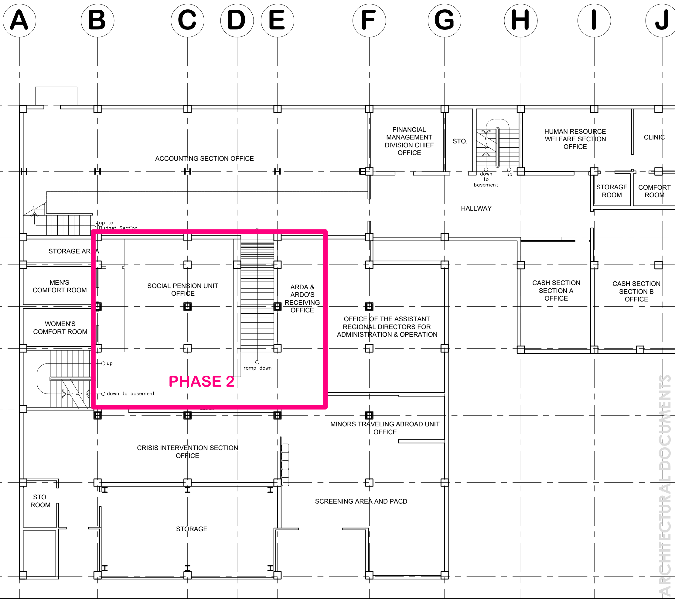
1 A 11 CONSTRUCTION PHASE 2 DEMARICATION PLAN SCALE 1:125 METERS
