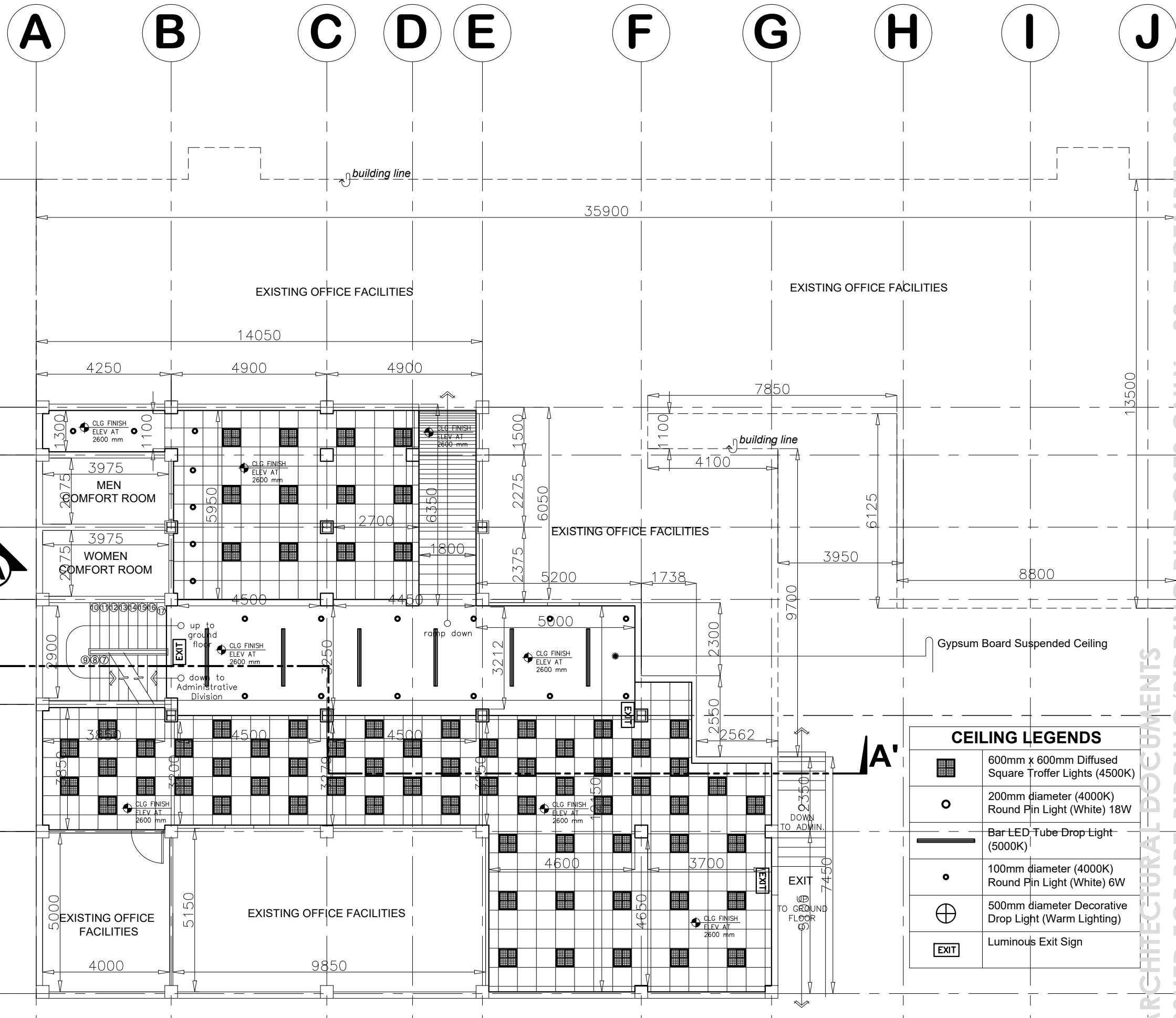
FIRST BASEMENT REFLECTED CEILING PLAN SCALE 1:125 METERS
