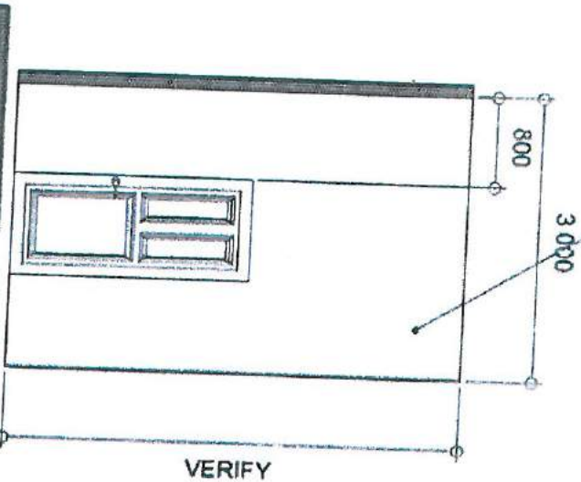
02 A 04 SCALE RIGHT SIDE ELEVATION NTS
